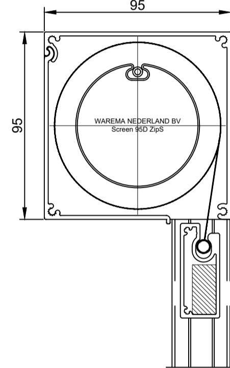
Screens 95D ZipS
