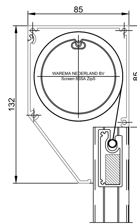
Screens 85SA ZipS
