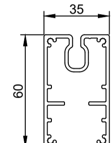
Bunnlist 35x60 mm
