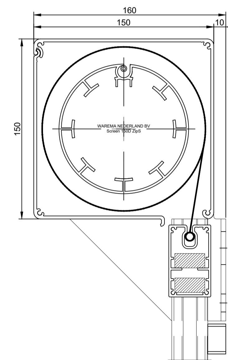
Screens 150D ZipS
