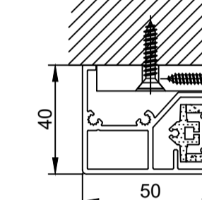
Styreskinne 40x50 mm single
