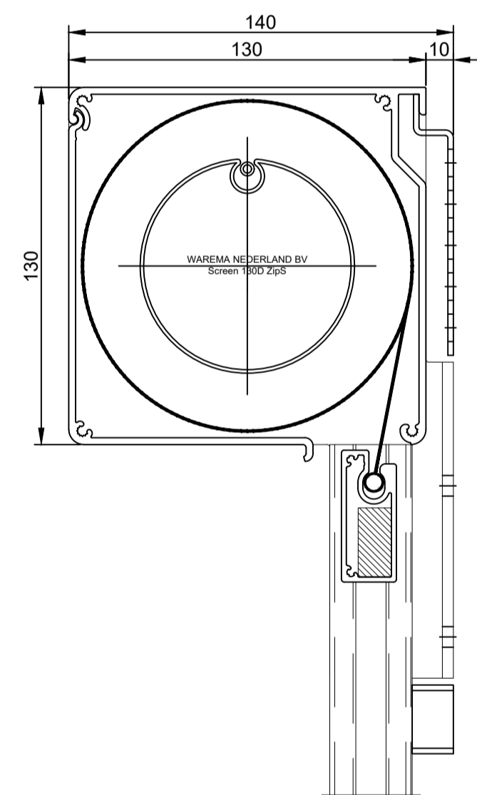
Screens 130D ZipS
