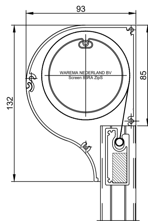
Screens 85RA ZipS
