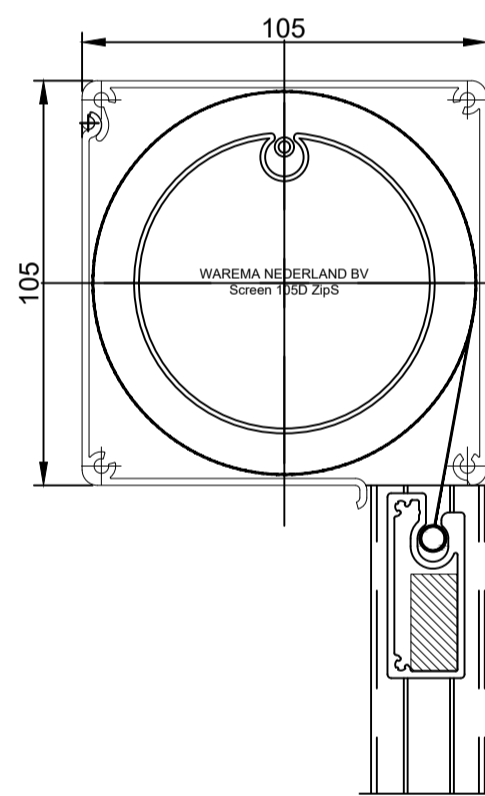
Screens 105D ZipS
