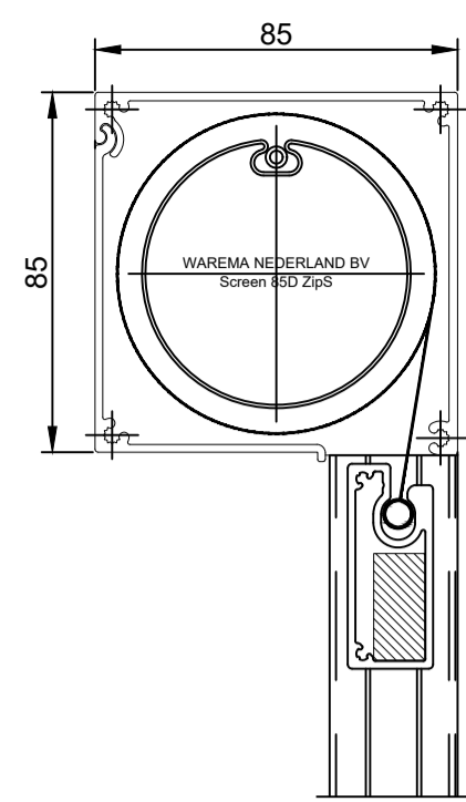
Screens 85D ZipS
