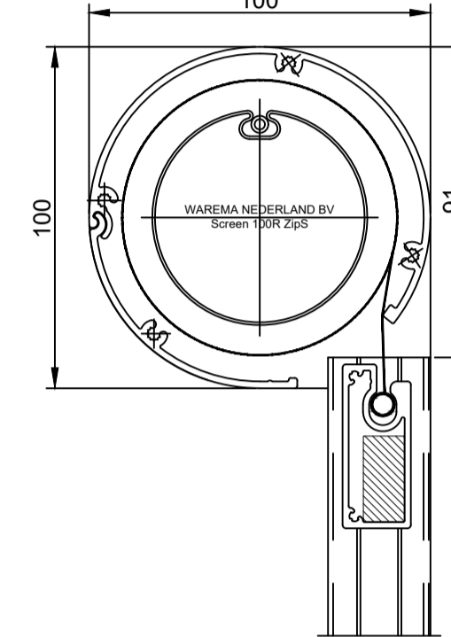
Screens 100R ZipS
