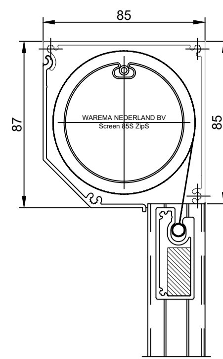
Screens 85S ZipS
