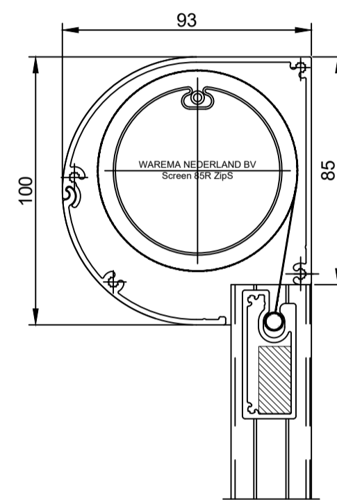
Screens 85R ZipS
