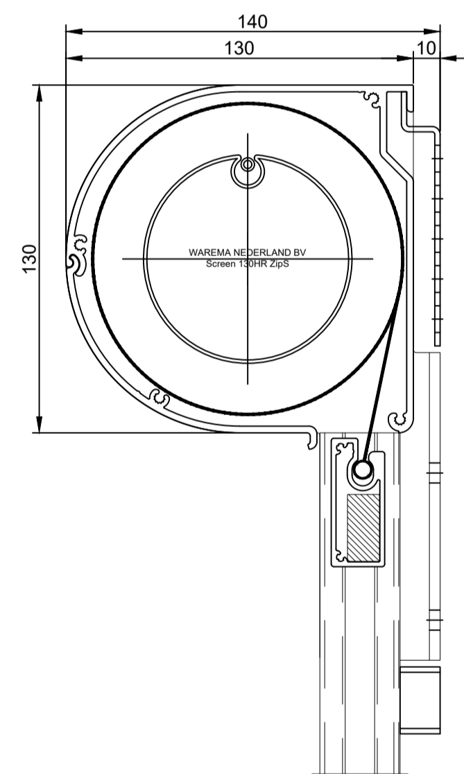
Screens 130HR ZipS
