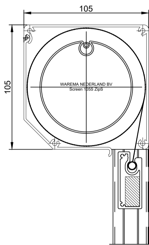
Screens 105S ZipS
