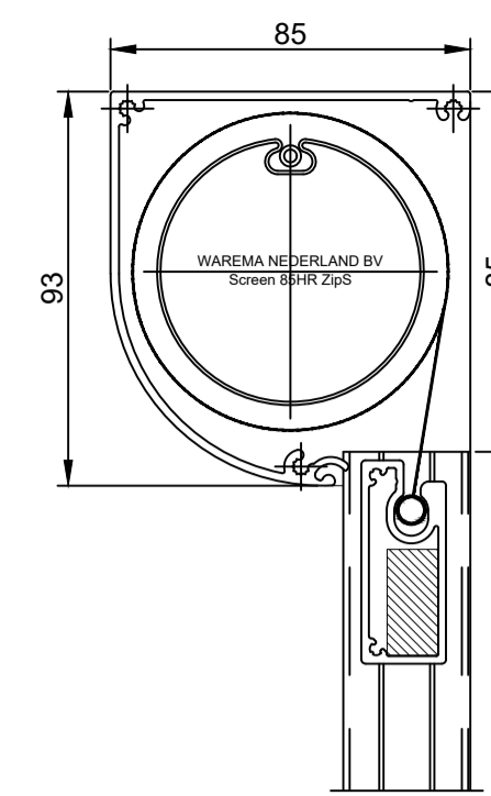
Screens 85HR ZipS
