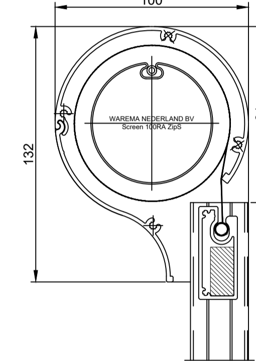
Screens 100RA ZipS
